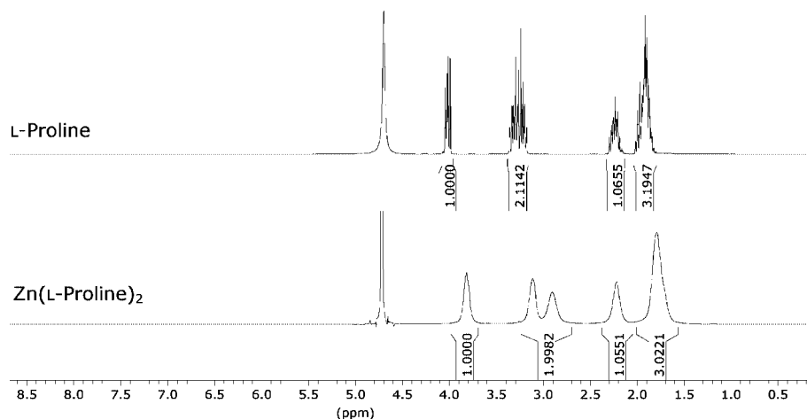
Figure 1. ^1\text{H} NMR spectrum of \text{Zn}(\text{Pro})_2 in \text{D}_2\text{O} compared with the spectrum of L-proline.
