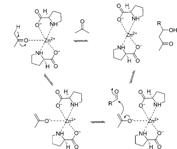
Figure 6. Proposed mechanism of the zinc–proline-catalyzed aldol reaction with zinc acting as Lewis acid.
