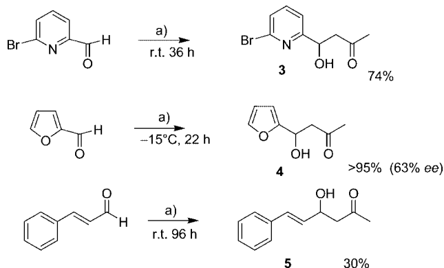
Figure 4. a): \text{Zn}(\text{Pro})_2 (5 mol-%), aldehyde (0.75 mmol), acetone (5 mL), water (10 mL).
