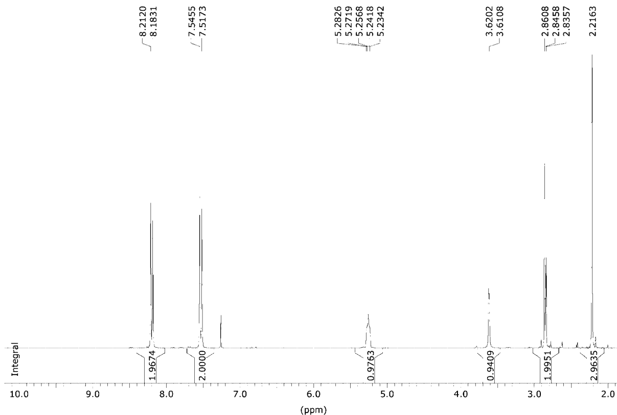
Figure 3. 1 H NMR spectrum (300 MHz, CDCl 3 ) of the crude product 2a from the aldol reaction of acetone and 1a after removal of the catalyst by filtration.
