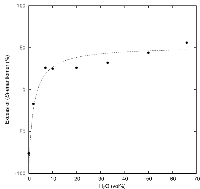
Figure 2. Excess of ( S ) enantiomer of 2a vs. H 2 O (vol%).
