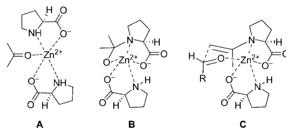
Figure 7. Proposed intermediates for the zinc-assisted enamine mechanism of the zinc–proline-catalyzed aldol reaction.
