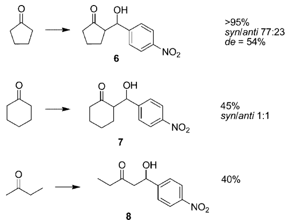
Figure 5. Aldol reaction with 1a catalyzed by \text{Zn}(\text{Pro})_2 . Conditions: 1a (1 mmol), ketone (4 mmol), \text{Zn}(\text{Pro})_2 (5 mol-%), THF (8 mL), water (8 mL), room temperature for 48 h.
